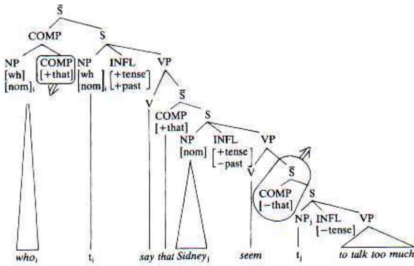
S-structure phrase marker for [246].
