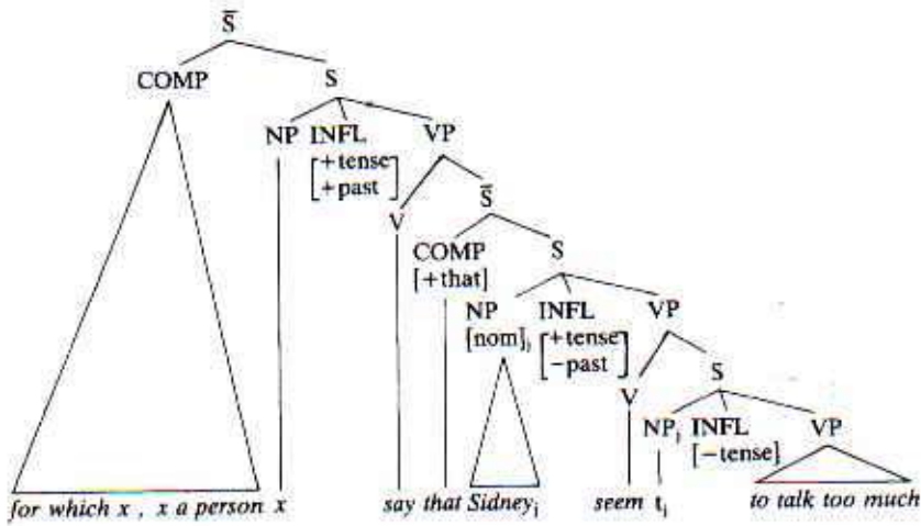
LF representation for [246].
